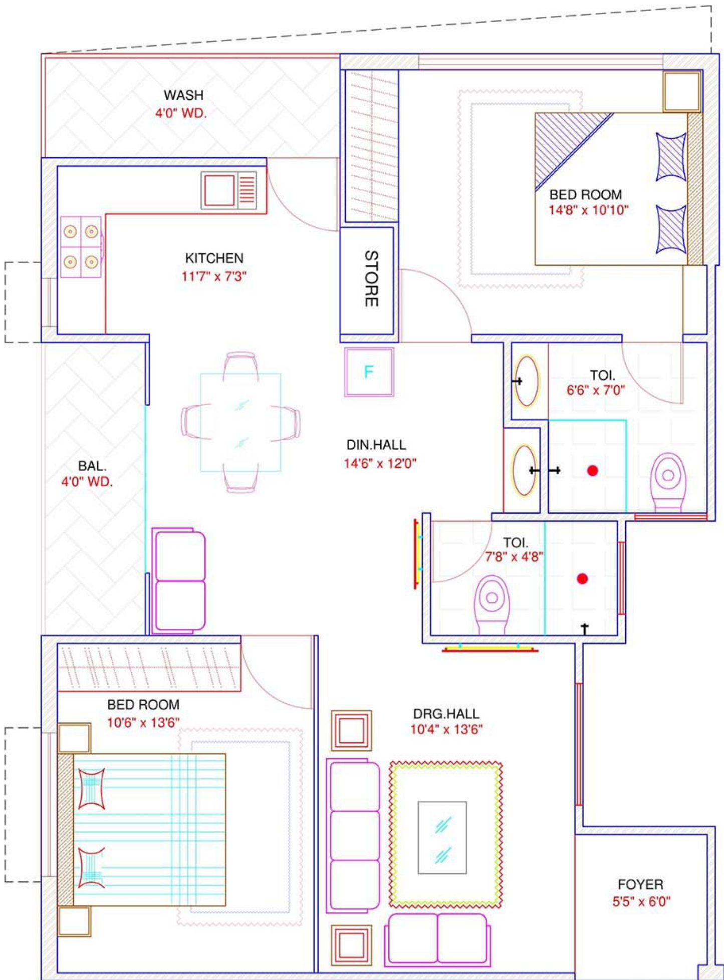
2 BHK PLAN ( TYPE 1 )
