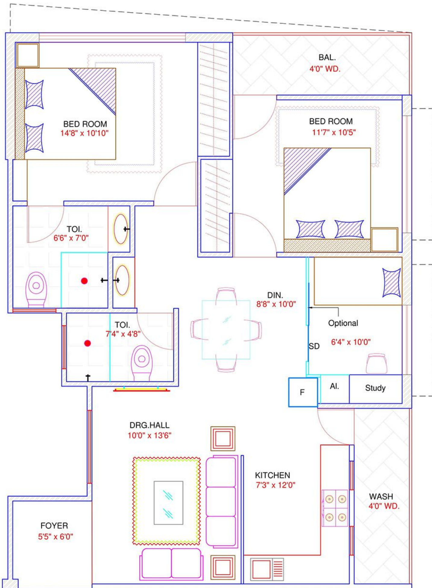
2.5 BHK PLAN ( TYPE 2 )
